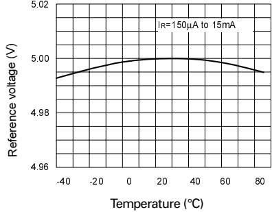
Temperature Drift
