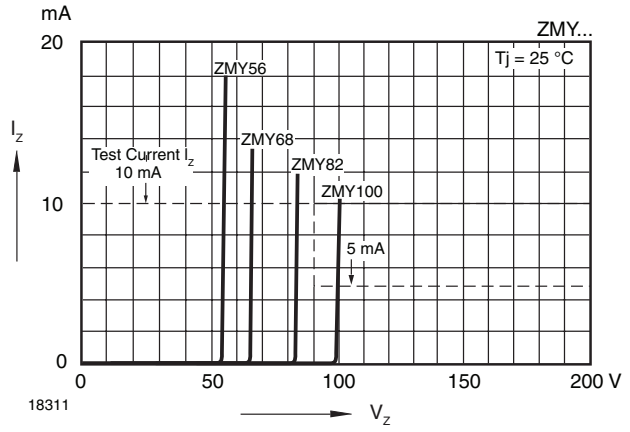
Figure 8. Breakdown Characteristics
