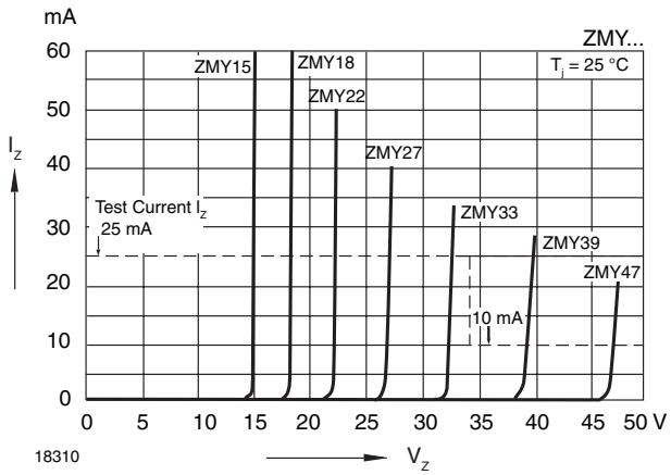
Figure 7. Breakdown Characteristics
