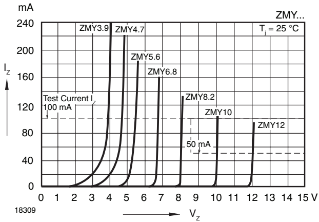
Figure 6. Breakdown Characteristics
