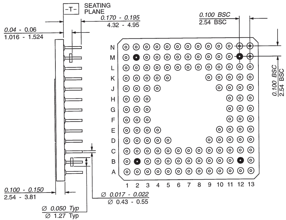
Figure 11-1. 132-ball-Ceramic Pin-Grid Array (PGA)
