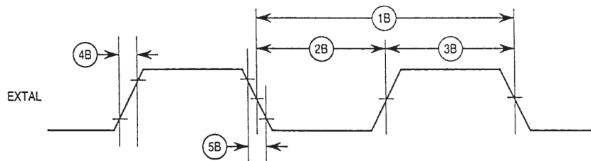
Figure 7-2. External Input Timing Diagram
