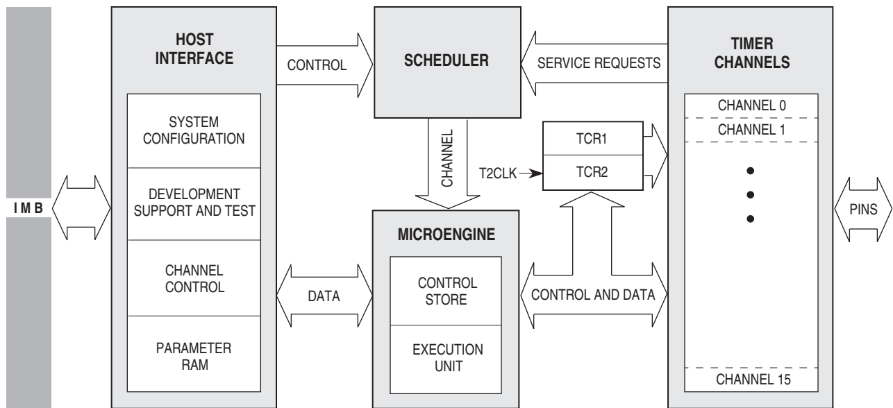
Figure 8-10. TPU Simplified Block Diagram
