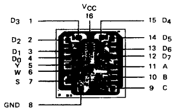
Am54S/74S151
