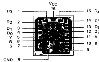
Am54S/74S251
