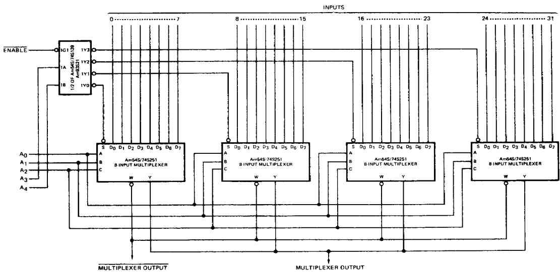
Am54S/74S251
