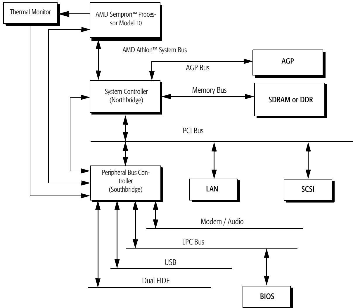
Figure 1. Typical AMD Sempron™ Processor Model 10 System Block Diagram
