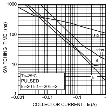
Fig.6 Switching time
