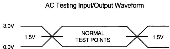
AC Test Point/Load Circuit Table
