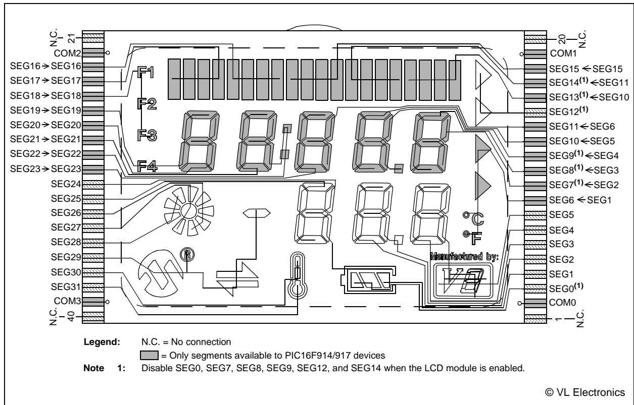
FIGURE A-9: SEGMENT CONFIGURATION FOR PIC16F914/917 DEVICES
