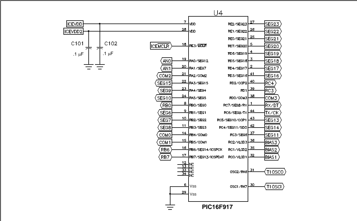
FIGURE A-20: PICDEM™ LCD 2 PIC16F914/917 PIM SCHEMATIC
