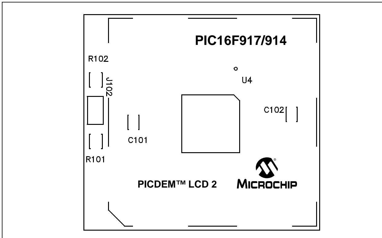
FIGURE A-16: PIC16F914/917 PIM LAYOUT
