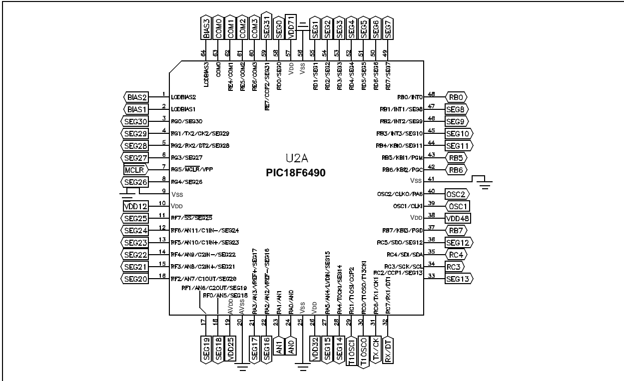
FIGURE A-22: PICDEM™ LCD 2 PIC18F6490 64-PIN PIM SCHEMATIC
