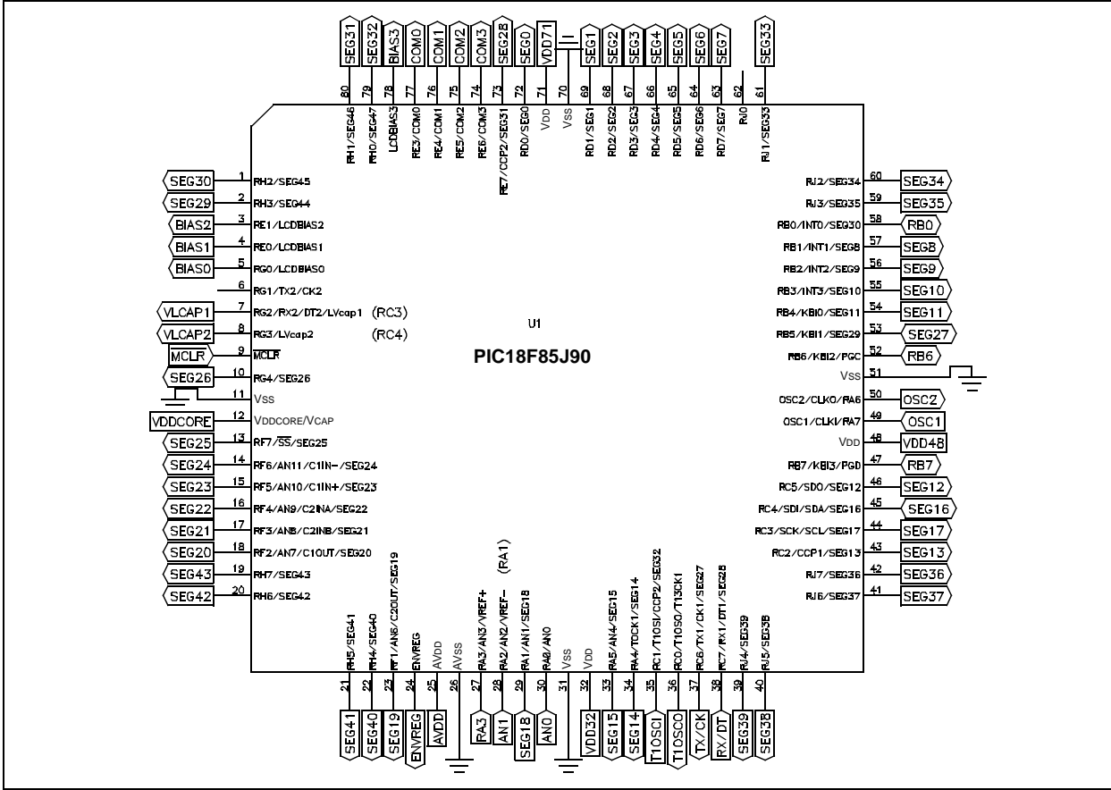
FIGURE A-26: PICDEM™ LCD 2 PIC18F85J90 80-PIN PIM SCHEMATIC
