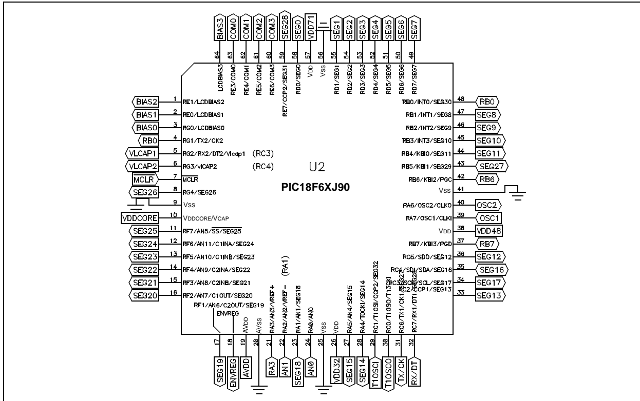
FIGURE A-24: PICDEM™ LCD 2 PIC18F6XJ90 64-PIN PIM SCHEMATIC
