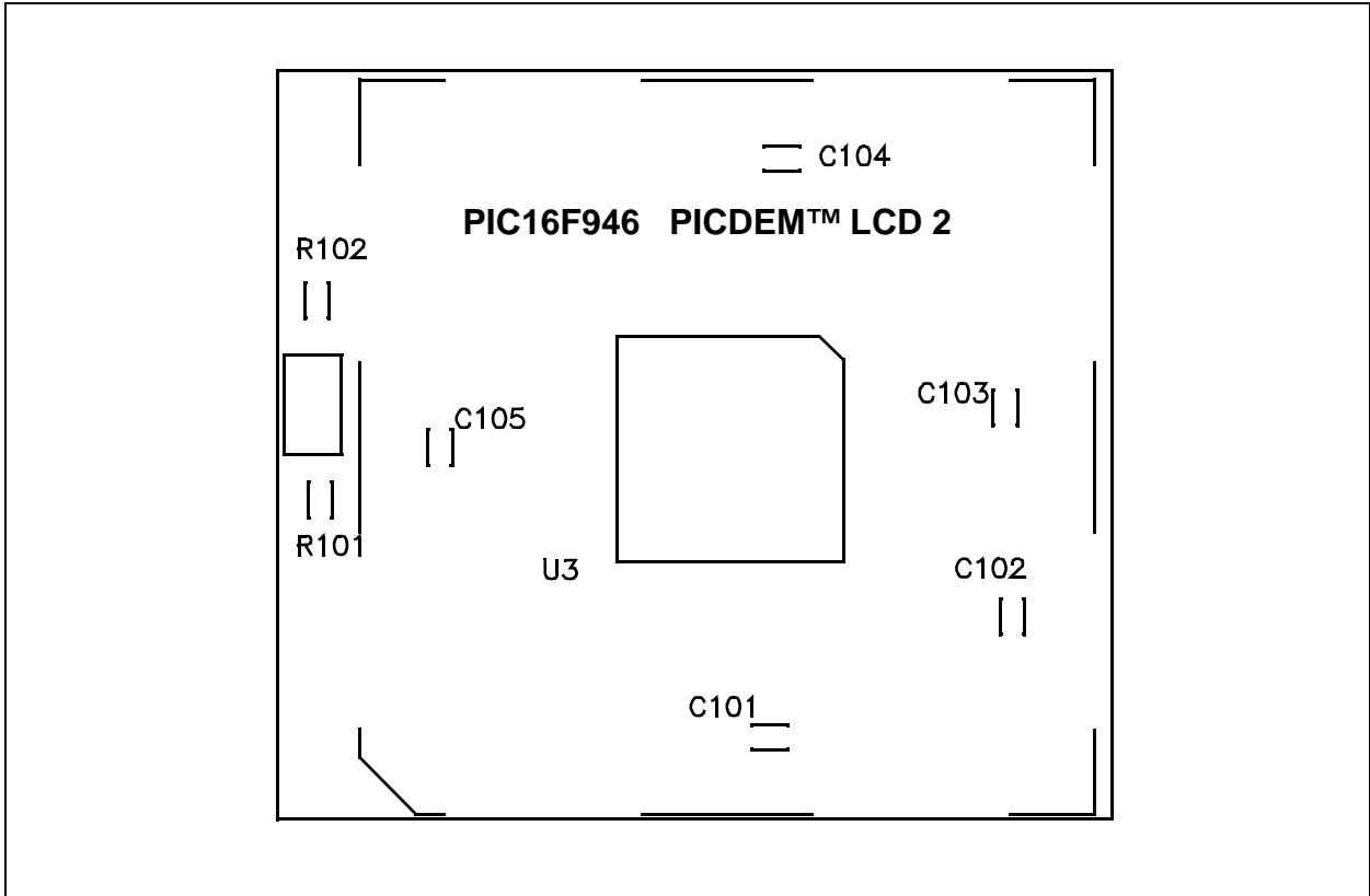
FIGURE A-17: PIC16F946 PIM LAYOUT
