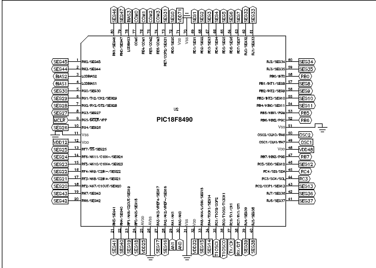
FIGURE A-23: PICDEM™ LCD 2 PIC18F8490 80-PIN PIM SCHEMATIC
