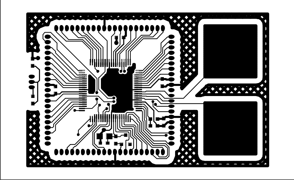
FIGURE A-19: PIC18F87J90 PIM LAYOUT
