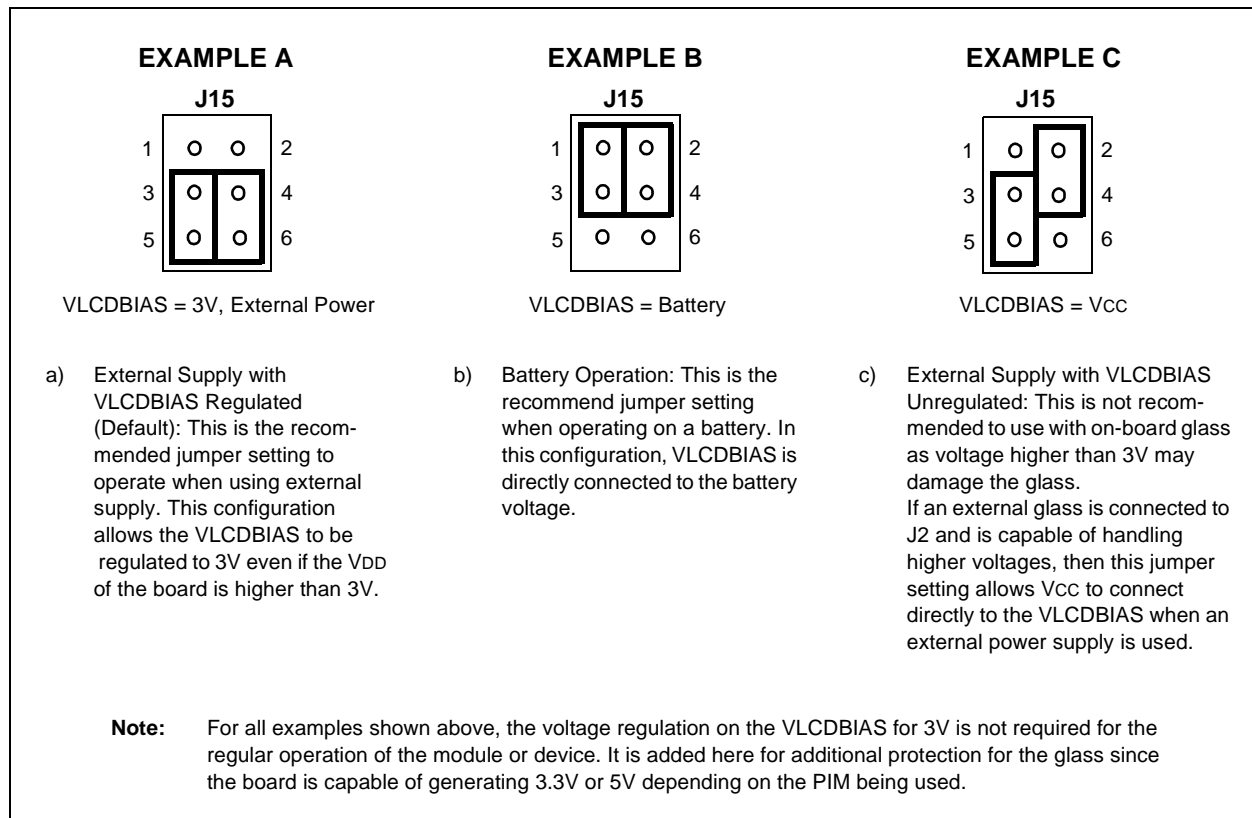
FIGURE A-10: J15 POWER SUPPLY CIRCUIT SETTING EXAMPLES
