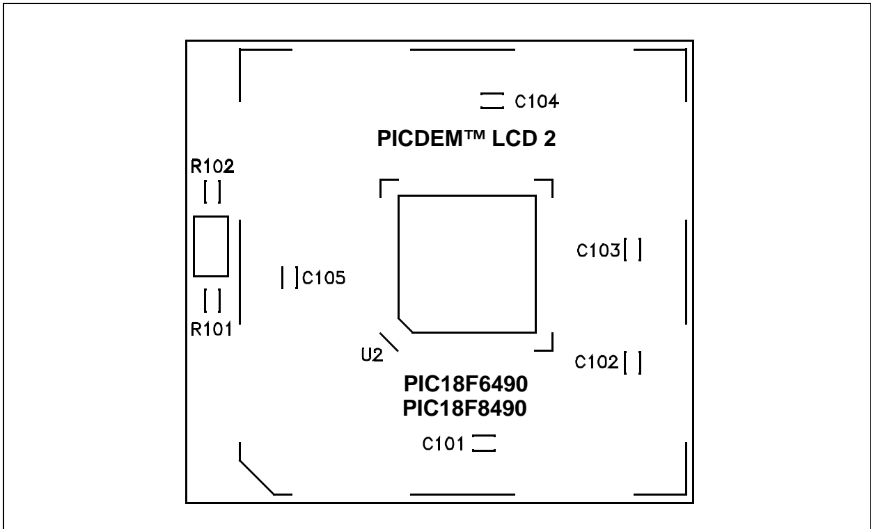
FIGURE A-18: PIC18F6490/8490 PIM LAYOUT
