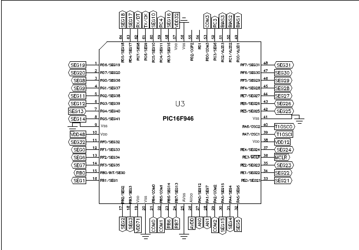
FIGURE A-21: PICDEM™ LCD 2 PIC16F946 PIM SCHEMATIC
