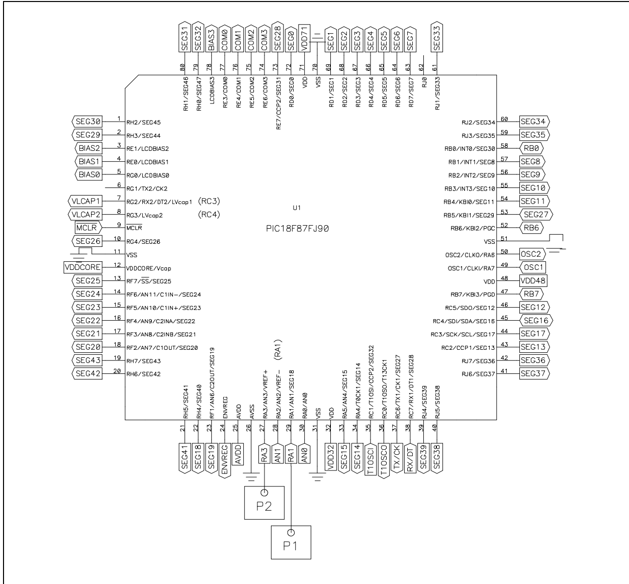
FIGURE A-25: PICDEM™ LCD 2 PIC18F87J90 80-PIN PIM SCHEMATIC
