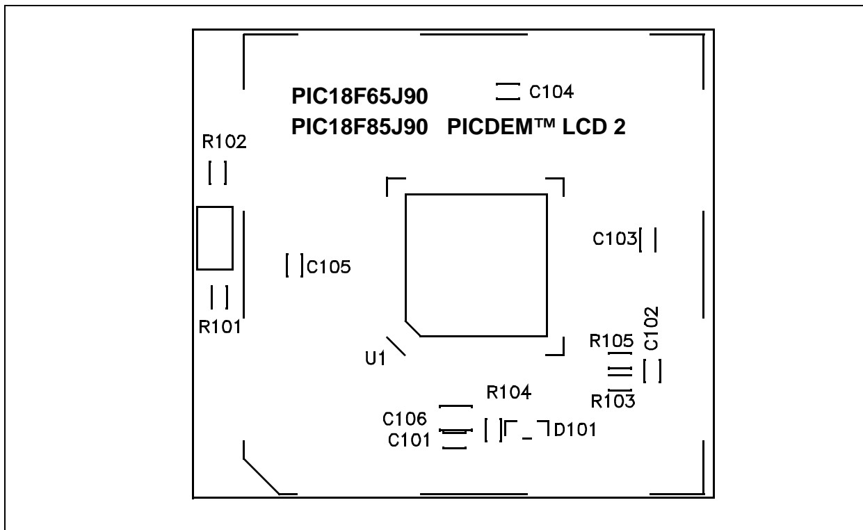
FIGURE A-15: PIC18F65J90 AND PIC18F85J90 PIM LAYOUT
