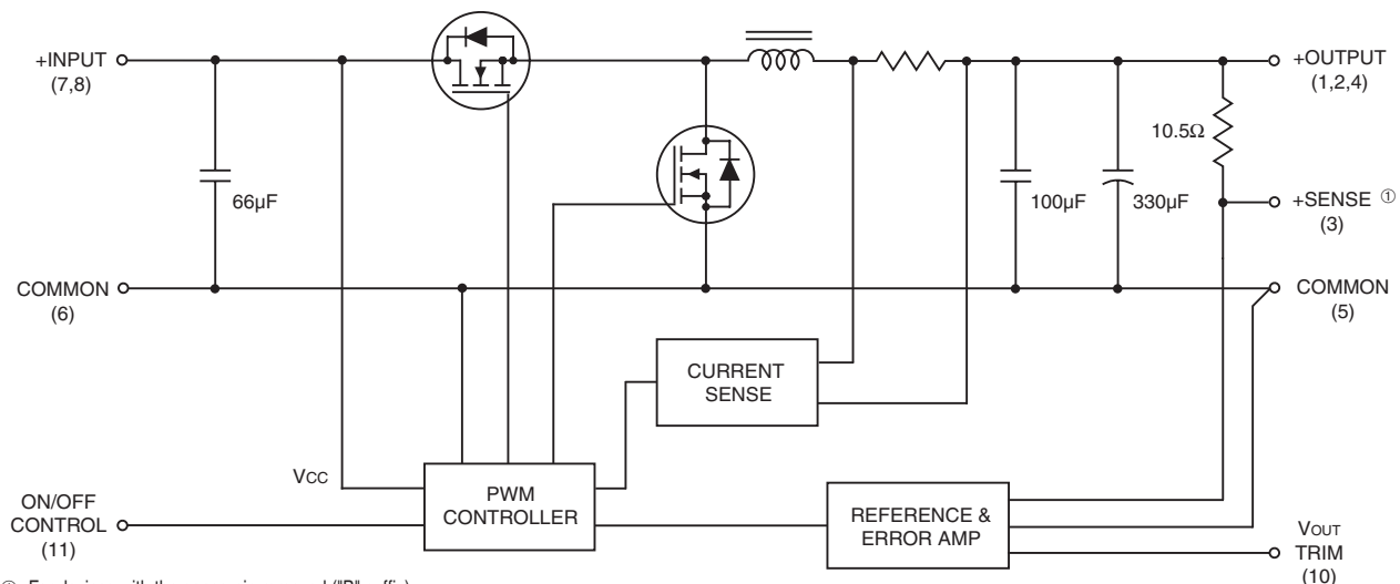
Figure 1. Simplified Schematic
