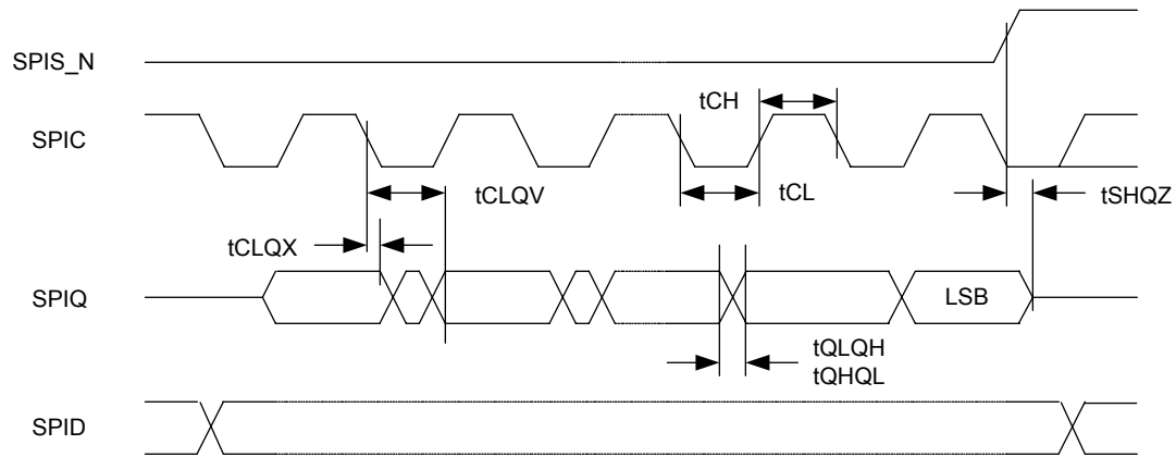
Figure 19. SPI Output Timing
