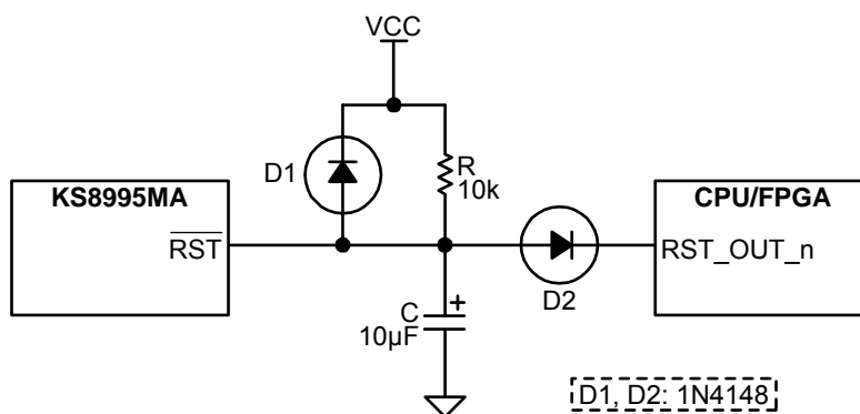
Figure 22. Recommended Circuit for Interfacing with CPU/FPGA Reset
