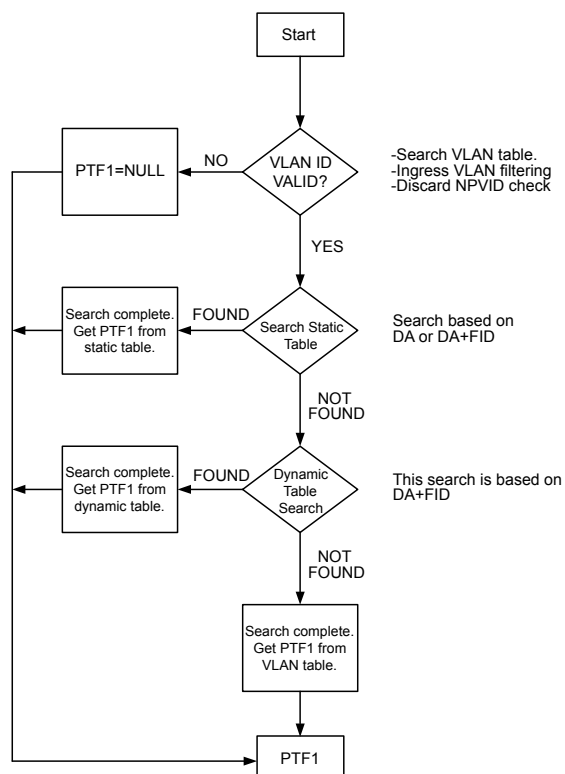
Figure 5. DA Look-Up Flowchart – Stage 1
