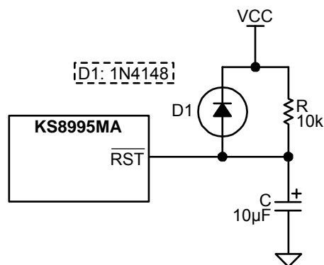
Figure 21. Recommended Reset Circuit
