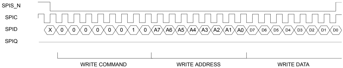
Figure 8. SPI Write Data Cycle
