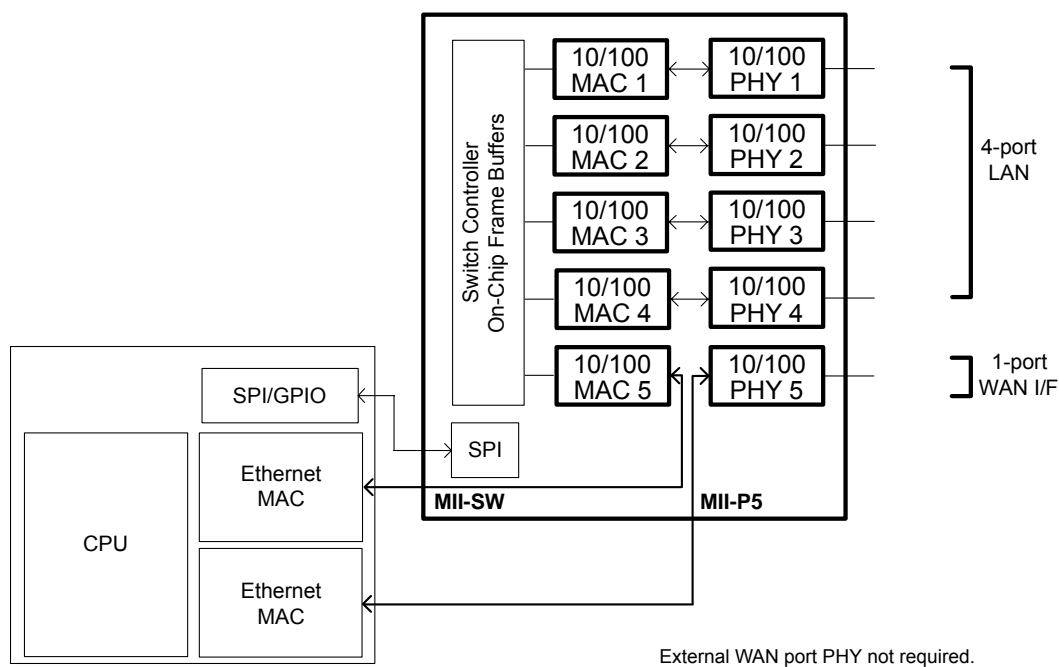
Figure 1. Broadband Gateway
