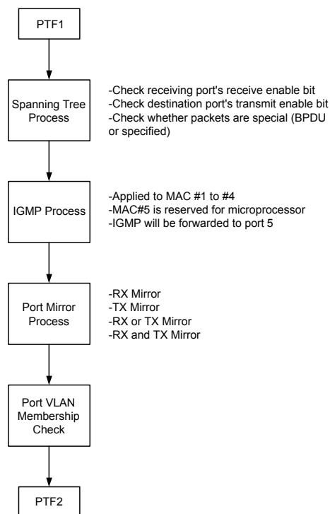
Figure 6. DA Resolution Flowchart – Stage 2
