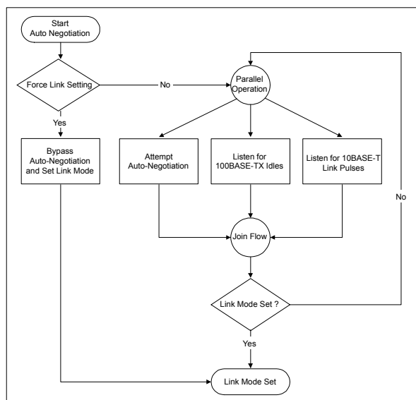
Figure 4. Auto-Negotiation
