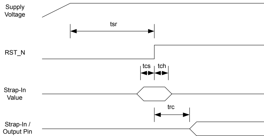
Figure 20. Reset Timing
