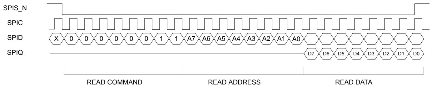
Figure 9. SPI Read Data Cycle
