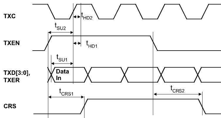
Figure 17. MII Transmitted Timing – For 100BASE-T
