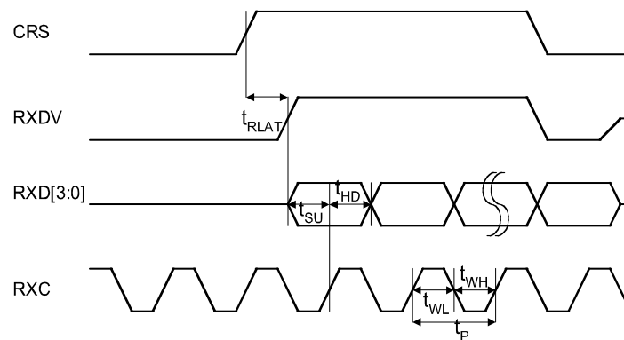
Figure 16. MII Received Timing – For 100BASE-T
