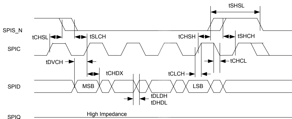
Figure 18. SPI Input Timing
