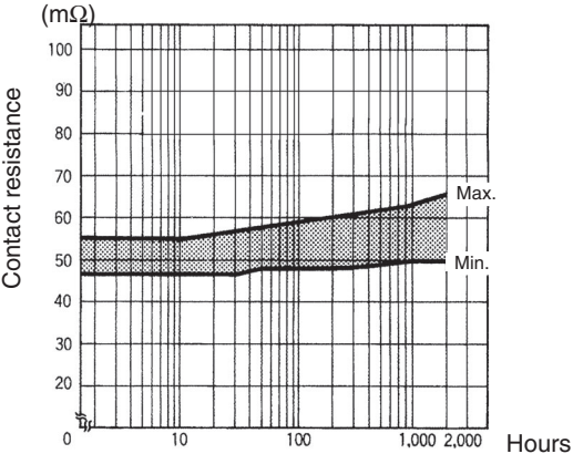
G2A-434A 24 VDC
