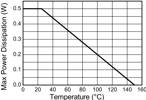
Derating Curve
