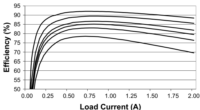
Efficiency vs. Load Current ( V_{in} = 5.0\text{V} )
