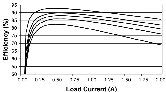
Efficiency vs. Load Current ( V_{in} = 3.3\text{V} )
