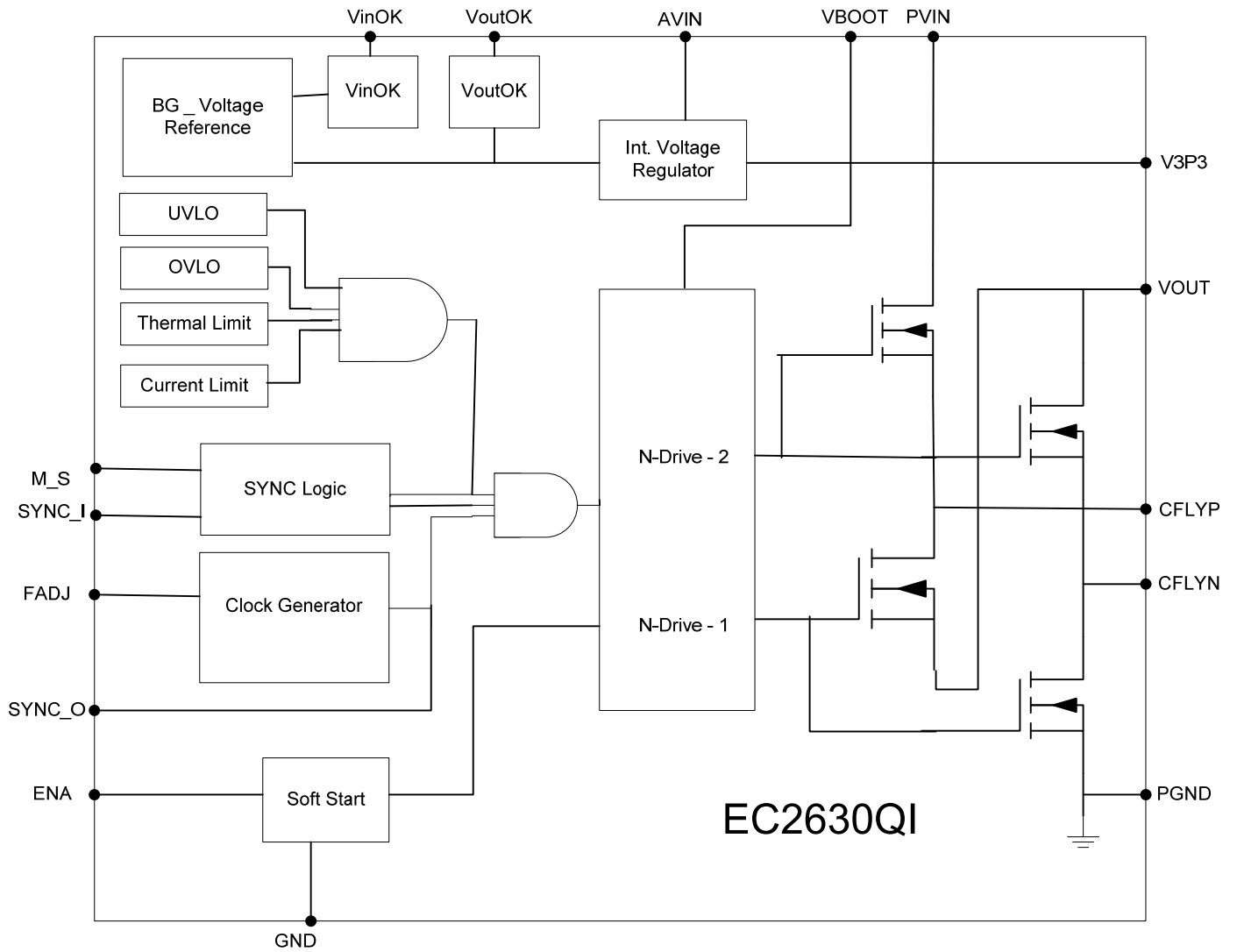
Figure 3: Block diagram.
