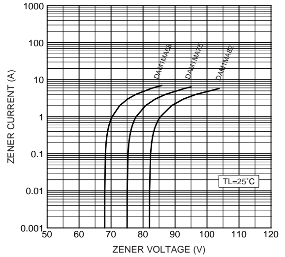
Typical zener characteristics ( Vz:68~82V)
