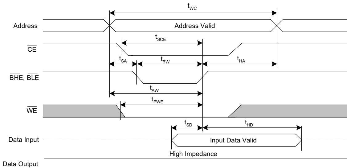
Figure 11. SRAM Write Cycle #3: \overline{\text{BHE}} and \overline{\text{BLE}} Controlled [3, 22, 23, 24, 25] (Not applicable for RTC register writes)
