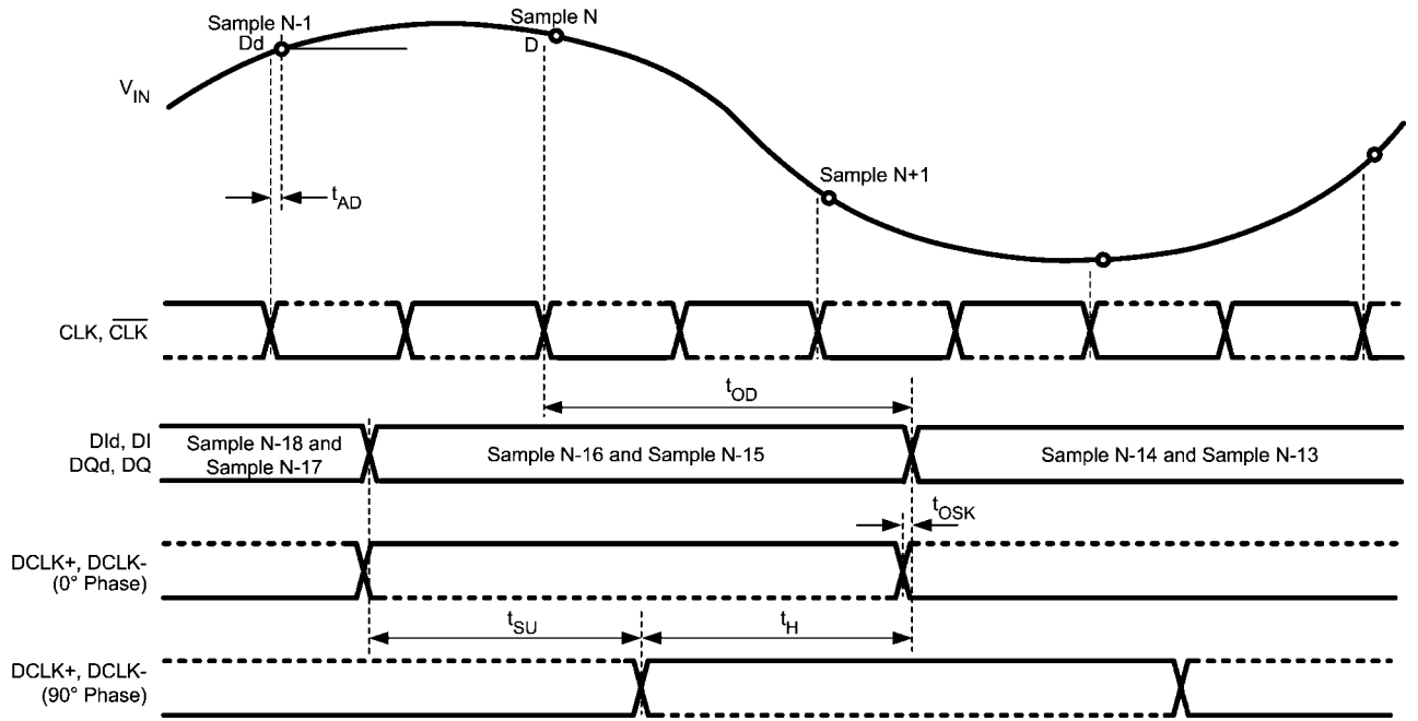
FIGURE 4. ADC08D500 Timing — DDR Clcking
