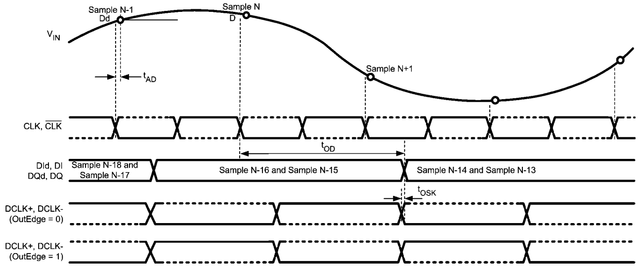
FIGURE 3. ADC08D500 Timing — SDR Clcking
