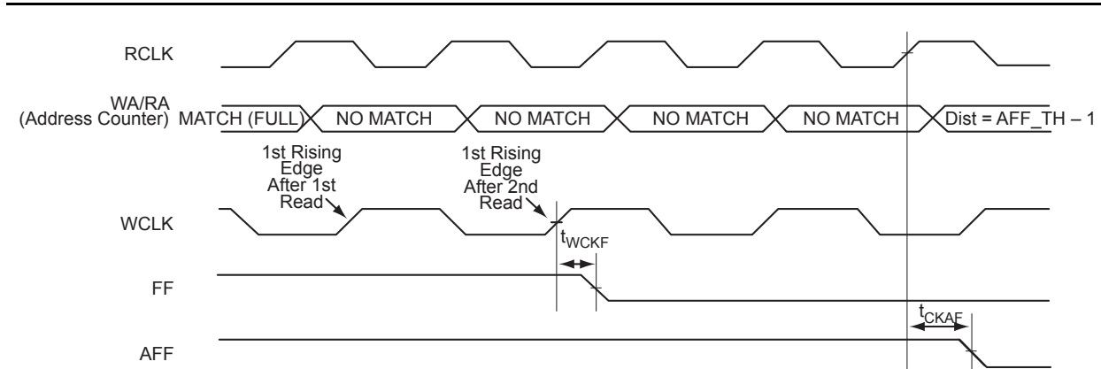
Figure 2-64 • FIFO FULL Flag and AFULL Flag Deassertion
