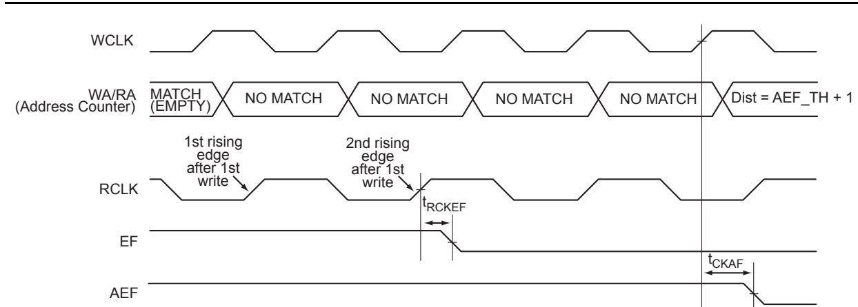
Figure 2-63 • FIFO EMPTY Flag and AEMPTY Flag Deassertion
