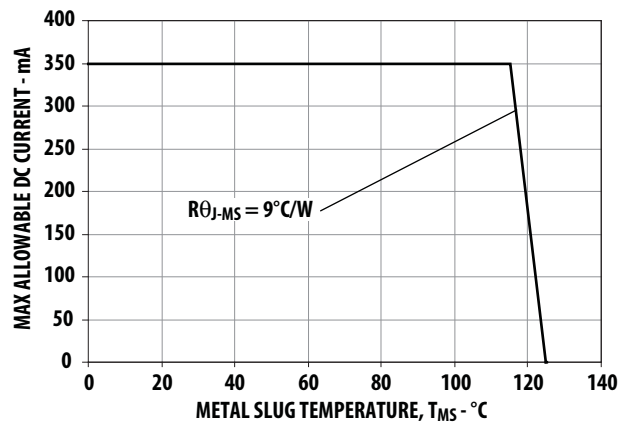
Figure 10. Maximum Forward Current vs. Ambient Temperature. Derated based on T_{JMAX} = 125^\circ\text{C} , R_{\theta J-MS} = 9^\circ\text{C/W}
