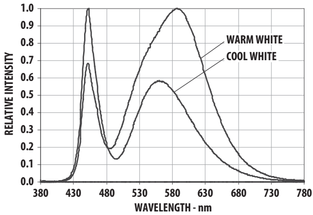
Figure 11. Relative Intensity vs. Wavelength for Cool and Warm White
