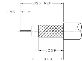
VIEW B
