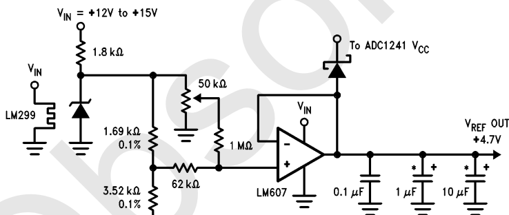
FIGURE 2. Low Drift Extremely Stable Reference Circuit
