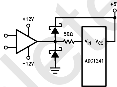
Protecting the Analog Inputs
