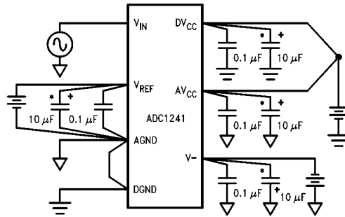
Power Supply Bypassing
