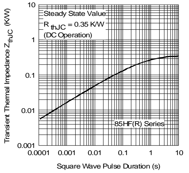
Fig. 12 - Thermal Impedance Z_{thJC} Characteristics
