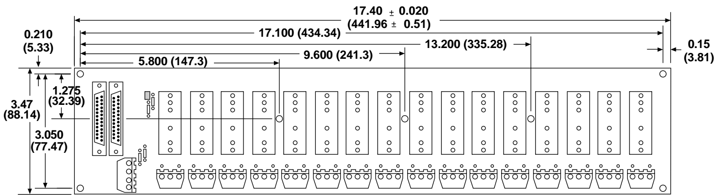
Model 7BP16-1 Backplane.
