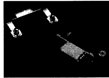
15-Position Receptacle, per VESA/VGA Standard with 4-40 Threaded Inserts or Female Screwlocks and Boardlocks, Blue Thermoplastic Housing
