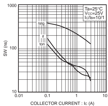
Fig.10 Switching Time
