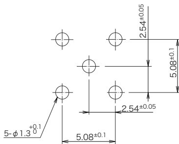
Panel Mounting Dimensions
