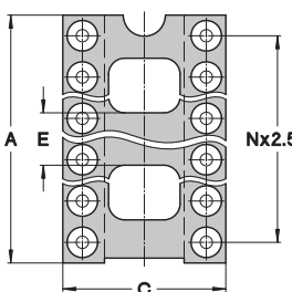
INSULATOR
