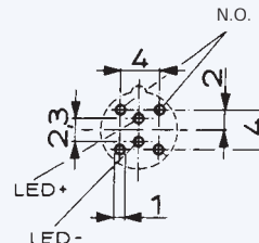
Drilling diagram
