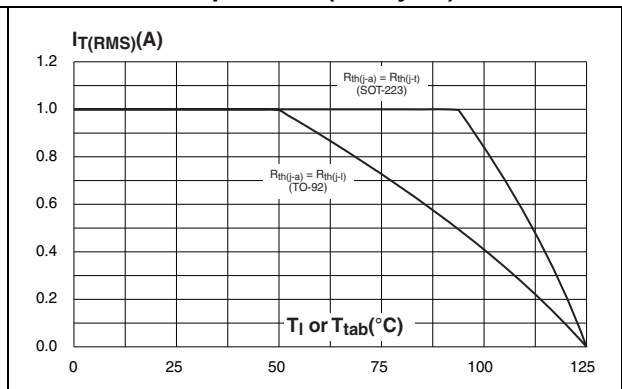
Figure 2. On-state rms current versus lead (TO-92) or tab (SOT-223) temperature (full cycle)
