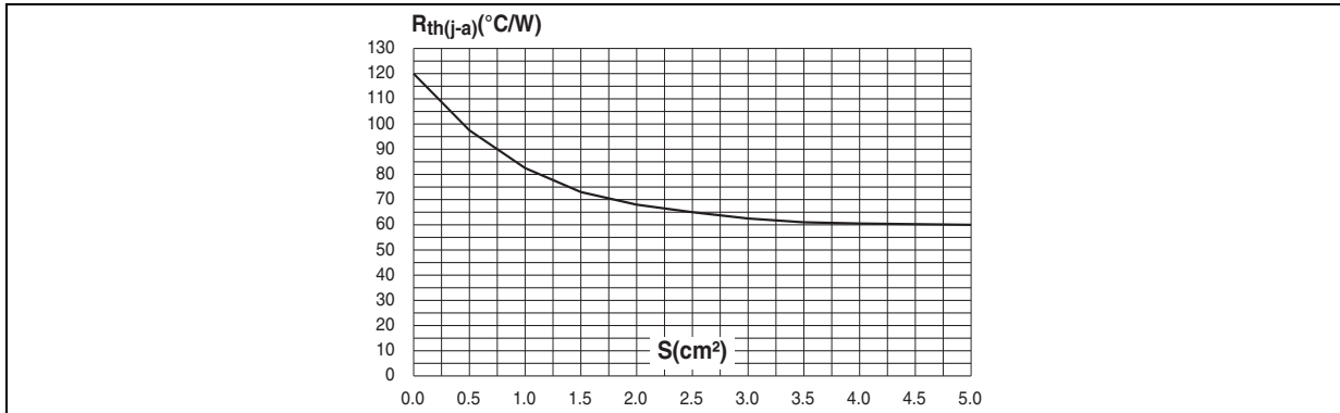
Figure 11. SOT-223 thermal resistance junction to ambient versus copper surface under case (printed circuit board FR4, copper thickness; 35 μm)
