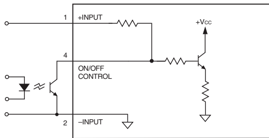
Figure 5. Driving the Negative Logic On/Off Control Pin
