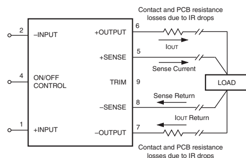
Figure 9. Remote Sense Circuit Configuration
