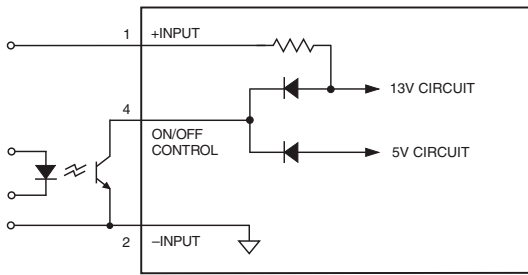
Figure 4. Driving the Positive Logic On/Off Control Pin
