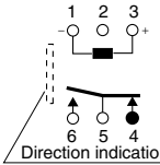
1-coil latching
