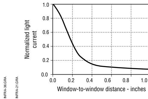
Fig. 6 Coupling Characteristics SE3450 with SD3443
