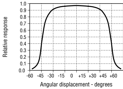
Fig. 1 Responsivity vs Angular Displacement (SD3443)
