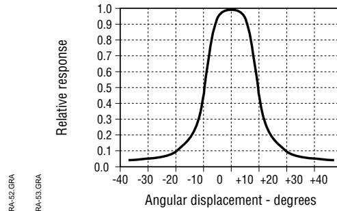
Fig. 2 Responsivity vs Angular Displacement (SD5443)
