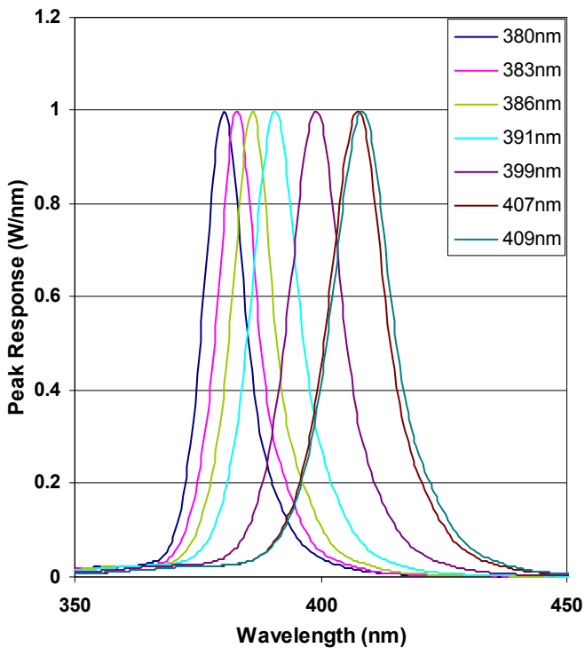
Normalized Peak Spectral Responses
