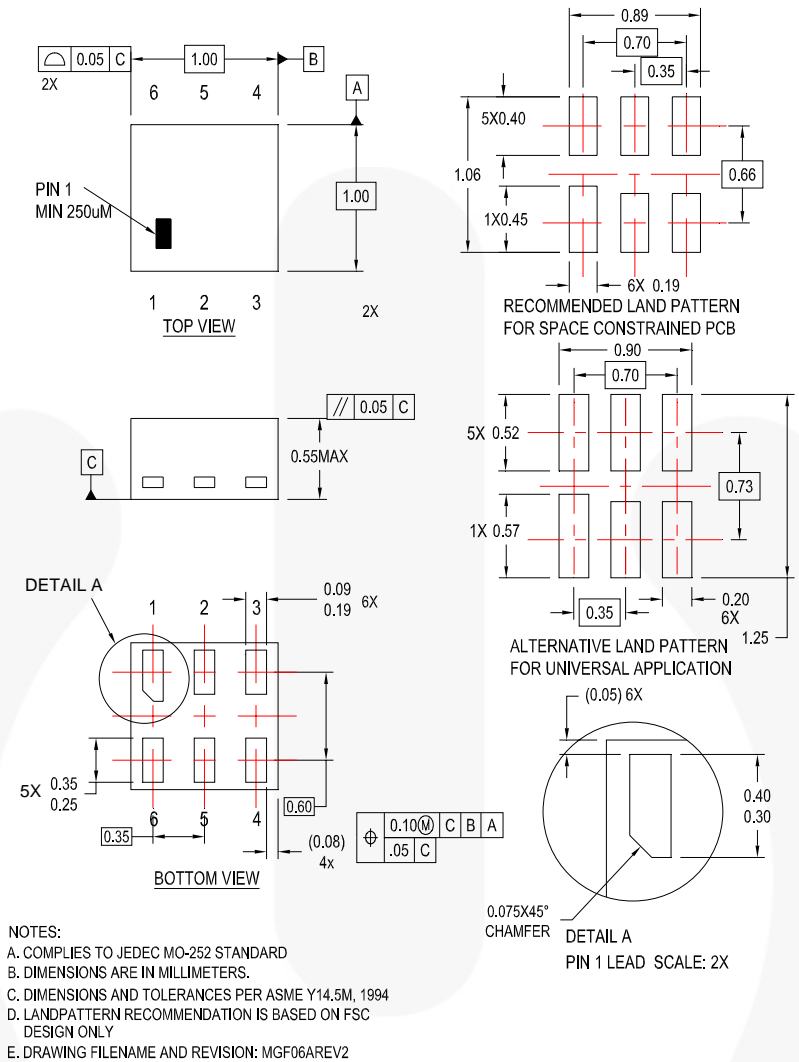
Figure 9. 6-Lead, MicroPak2, 1x1mm Body, .35mm Pitch
