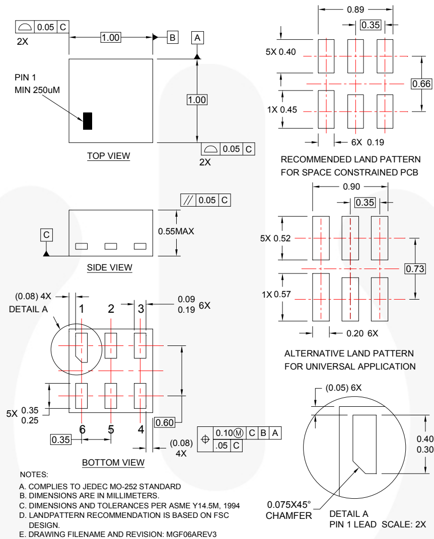
Figure 8. 6-Lead, MicroPak™, 1.0mm Wide
