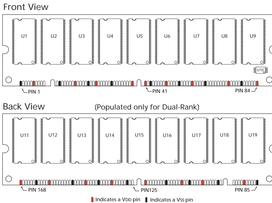
Figure 2: 168-Pin DIMM Pin Locations
