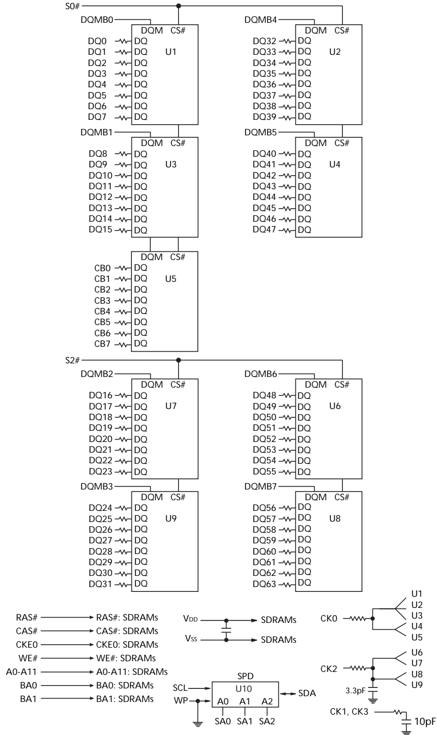
Figure 3: Functional Block Diagram – Single Rank
