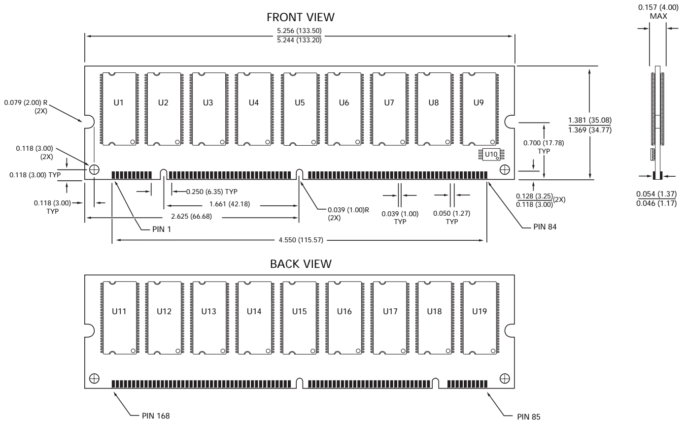
Figure 12: 168-Pin DIMM Dimensions - Dual-Rank
