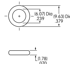
AT401P O-ring for Splashproof Models Natural Rubber
