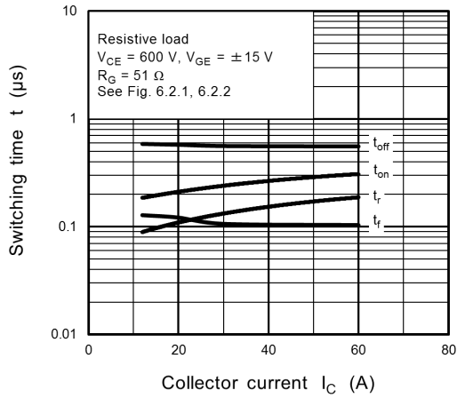
Fig. 8.7 Switching Time - I_C
