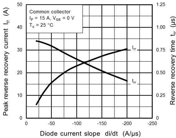
Fig. 8.15 I_{rr}, t_{rr} - di/dt
