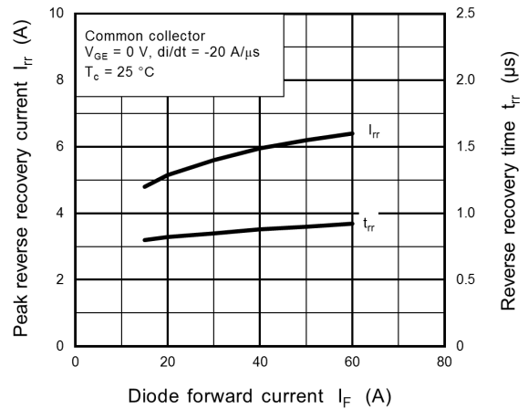
Fig. 8.16 I_{rr}, t_{rr} - I_F
