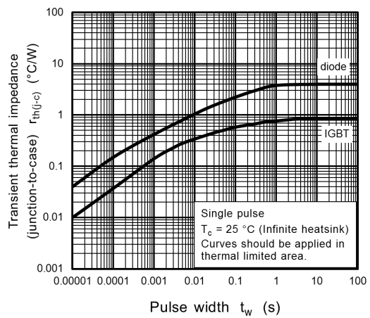
Fig. 8.12 r_{th(j-c)} - t_w (Guaranteed Maximum)
