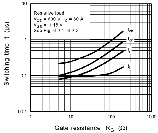
Fig. 8.8 Switching Time - R_G
