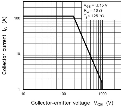
Fig. 8.13 Reverse Bias SOA (Guaranteed Maximum)
