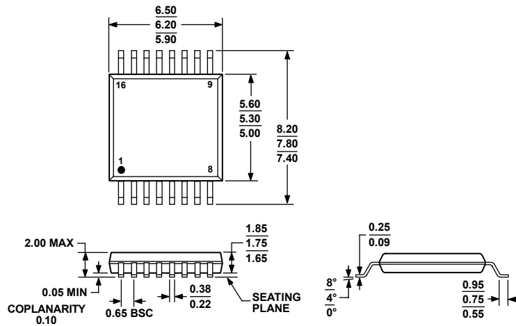
Figure 44. 16-Lead Shrink Small Outline Package [SSOP] (RS-16)
