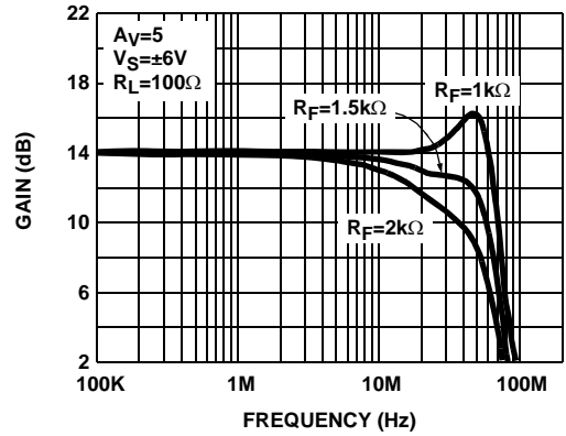
FIGURE 4. DIFFERENTIAL FREQUENCY RESPONSE vs R_F (EL1509CL)
