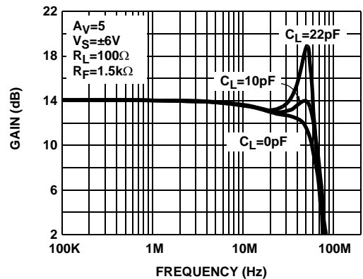
FIGURE 6. DIFFERENTIAL FREQUENCY RESPONSE vs C_L (EL1509CL)
