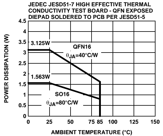
FIGURE 50. PACKAGE POWER DISSIPATION vs AMBIENT TEMPERATURE
