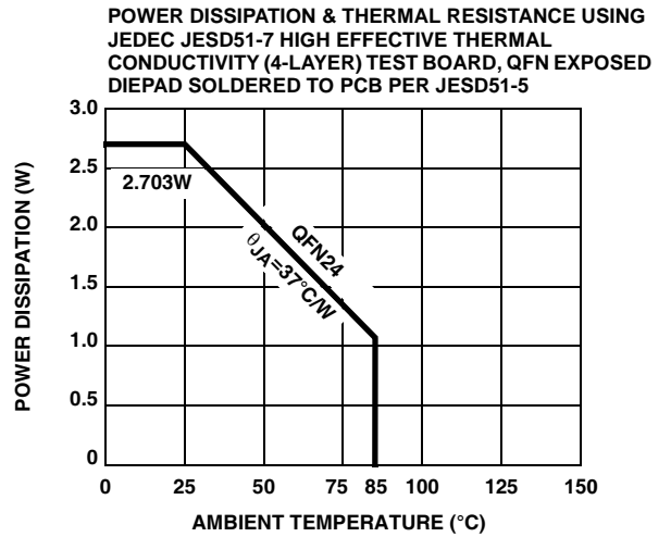
FIGURE 38. POWER DISSIPATION vs AMBIENT TEMPERATURE
