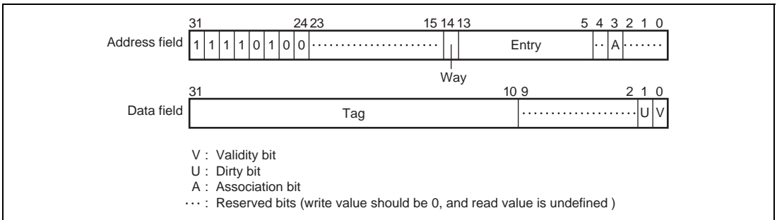
Figure 7.11 Memory-Mapped OC Address Array
