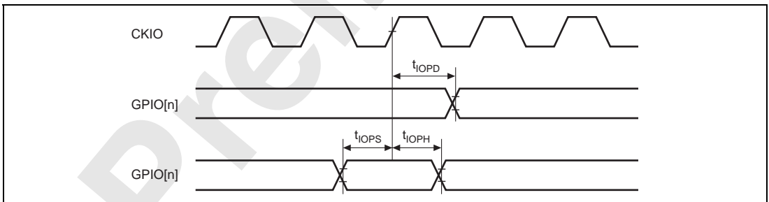
Figure 33.61 GPIO Timing
