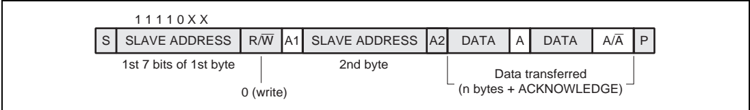
Figure 19.6 10-Bit Address Data Transfer Format
