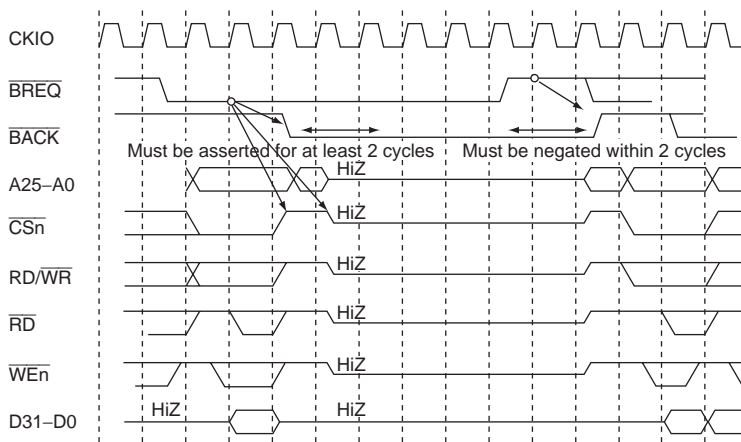
Figure 10.61 Arbitration Sequence
