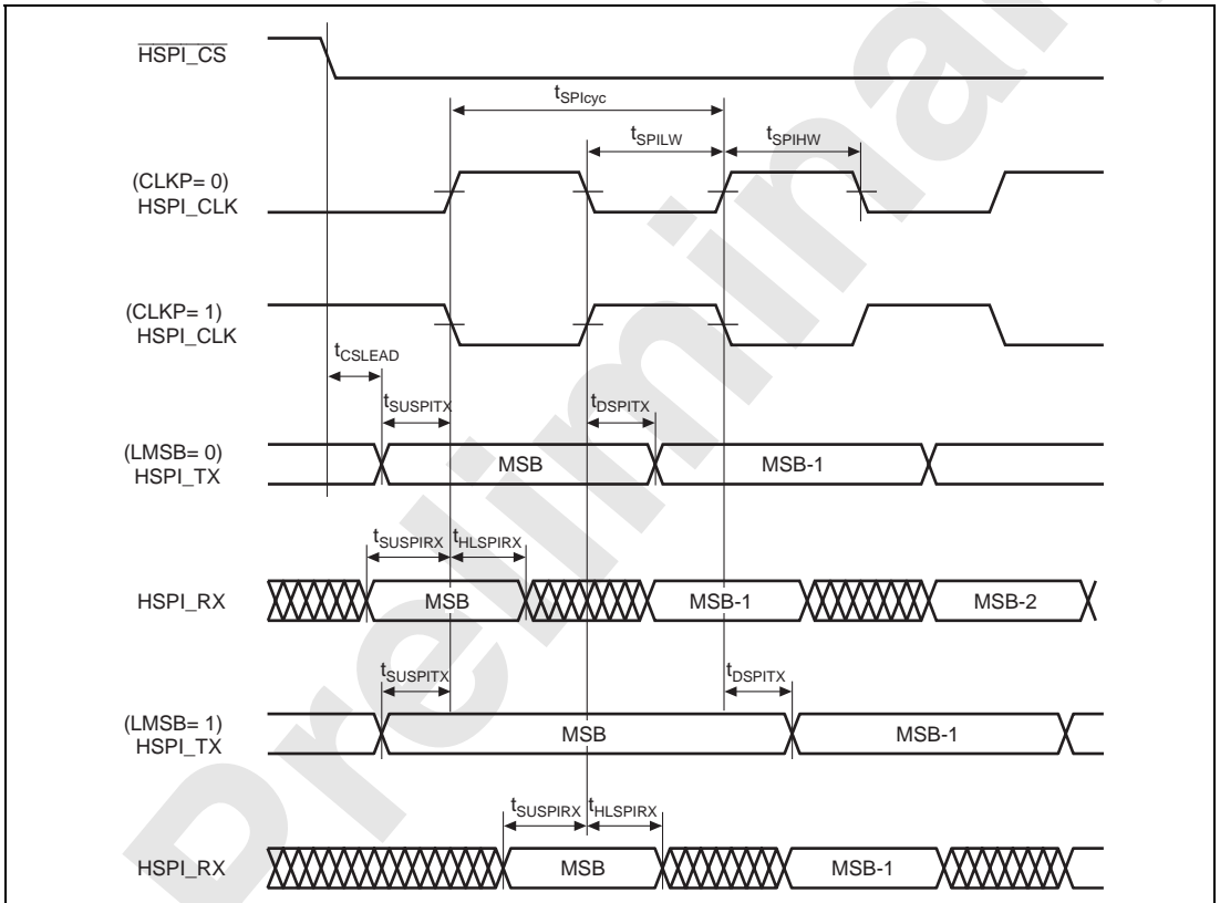
Figure 33.64 HSPI Data Output/Input Timing
