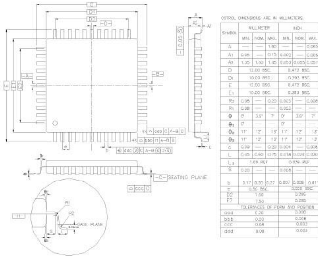
Figure 7-3: Low-profile Quad Flat Pack (LQFP), 64-pin
