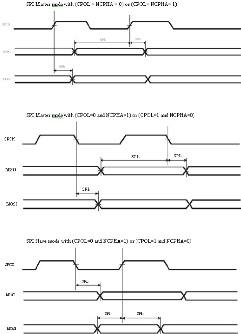
Figure 8-2: SPI Parameters
