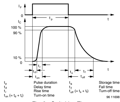
Fig. 3 - Switching Times
