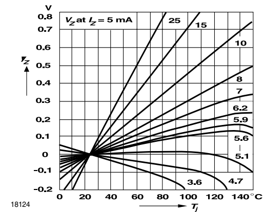
Figure 11. Change of Zener Voltage vs. Junction Temperature
