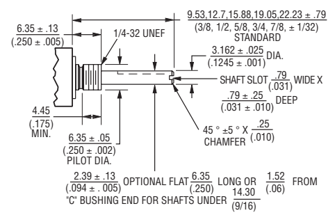
"C" Bushing 1/4 " (6.35 mm) Dia. Plain - Single Shaft
