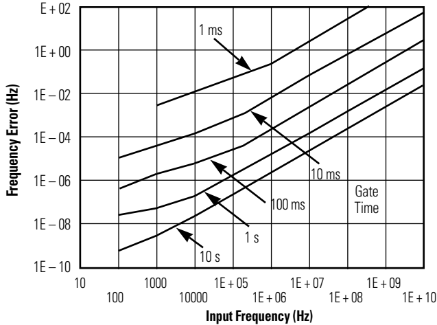
Graph 5: HP 53132A - Worst Case RMS Resolution 7 (Time or Digits Arming)
