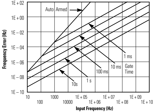
Graph 4: HP 53132A - Worst Case RMS Resolution 7 (Automatic or External Arming)
