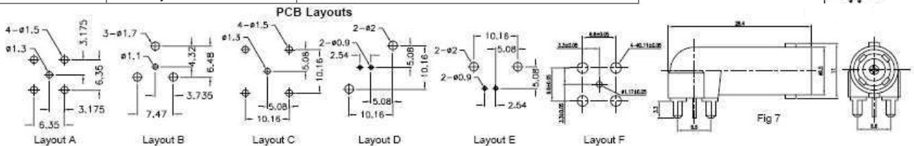
PCB Layouts
