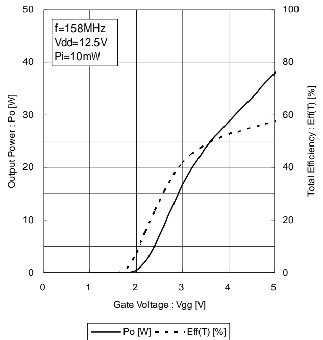
Output Power, Total Efficiency versus Gate Voltage
